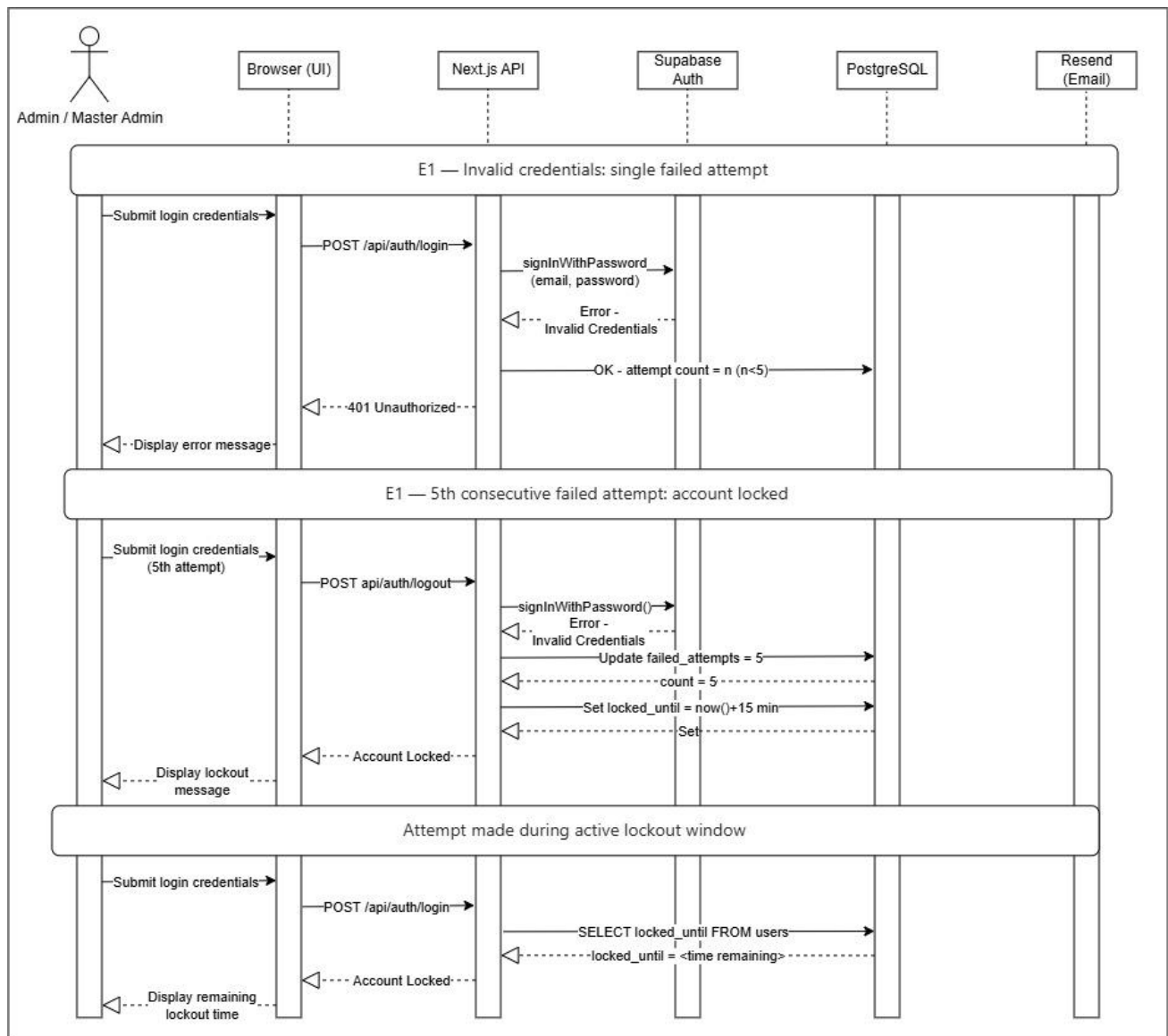
Figure 3.1.3 – User Access &amp; Account Management Exception Flow Sequence Diagram
