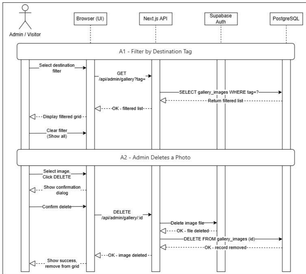
Figure 3.4.2 – Manage Gallery Alternative Flow Sequence Diagram
