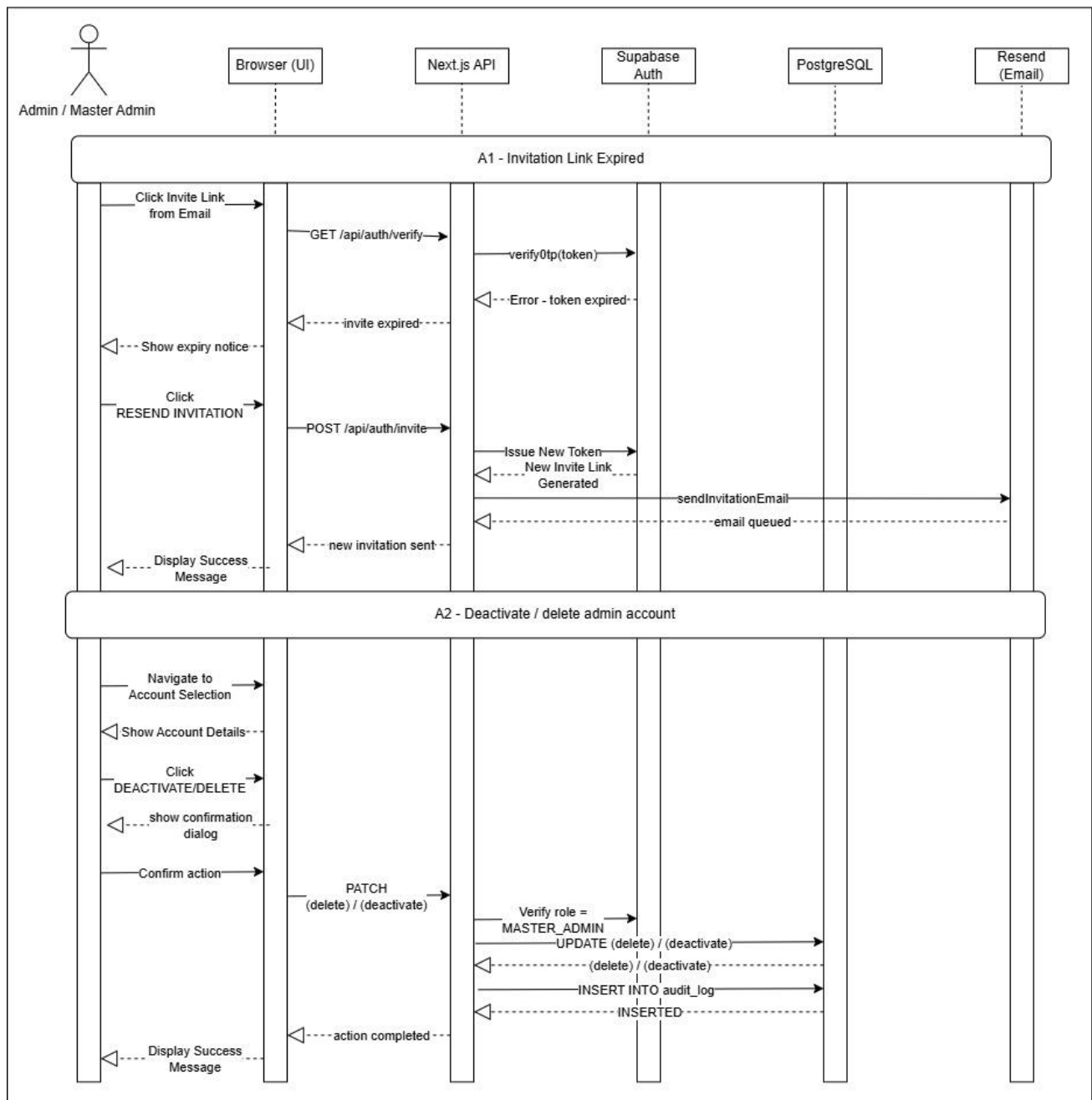
Figure 3.1.2 – User Access &amp; Account Management Alternative Flow Sequence Diagram
