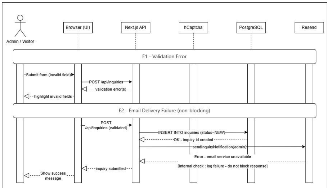
Figure 3.3.3 – Manage Inquiries Exception Flow Sequence Diagram
