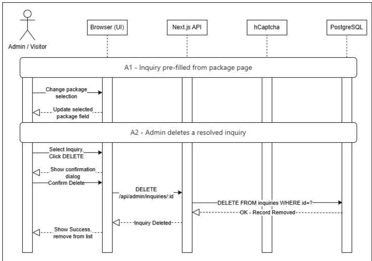
Figure 3.3.2 – Manage Inquiries Alternative Flow Sequence Diagram
