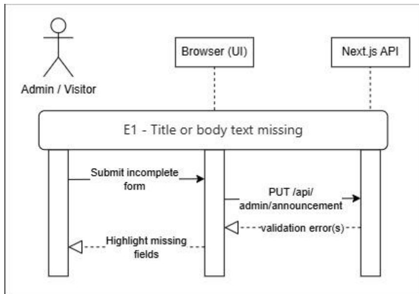
Figure 3.7.3 – Manage Announcements &amp; Promotions Exception Flow Sequence Diagram
