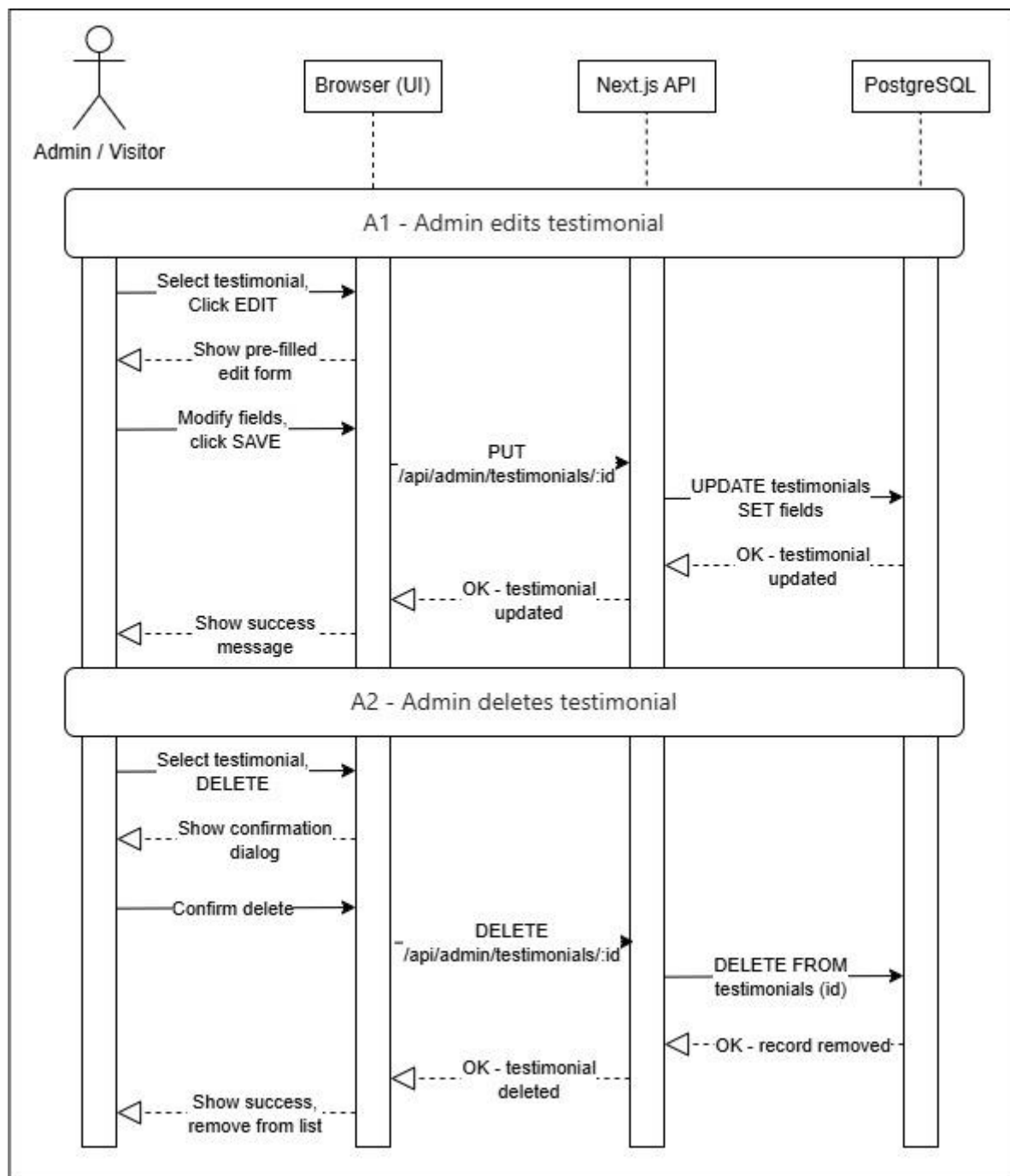
Figure 3.5.2 – Manage Testimonials Alternative Flow Sequence Diagram
