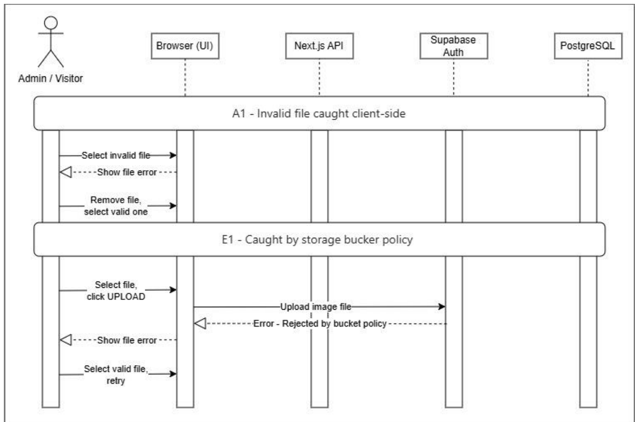
Figure 3.4.3 – Manage Gallery Exception Flow Sequence Diagram
