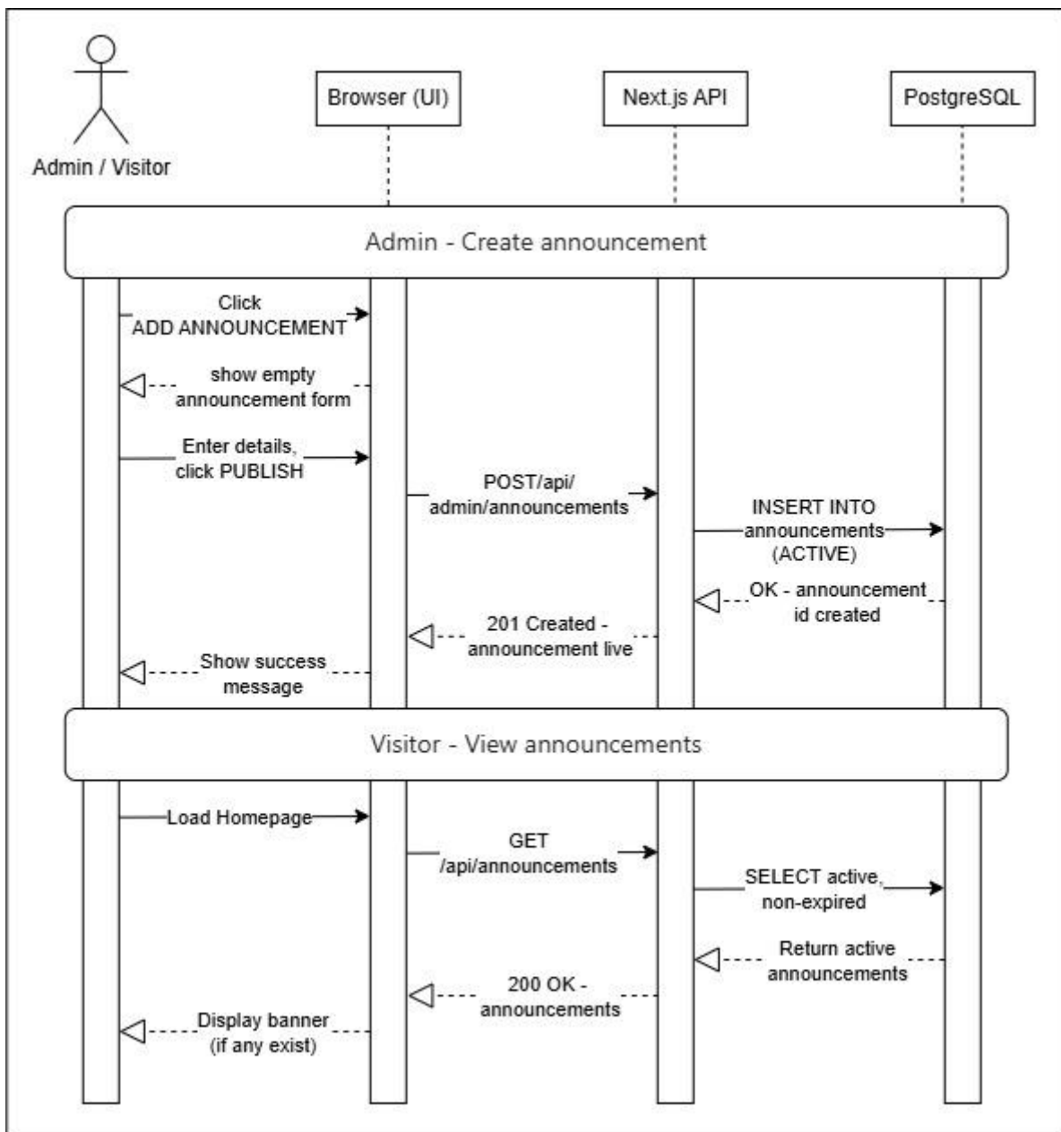
Figure 3.7.1 – Manage Announcements & Promotions Basic Flow Sequence Diagram
