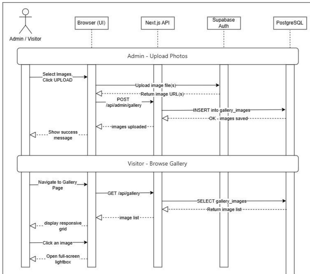
Figure 3.4.1 – Manage Gallery Basic Flow Sequence Diagram
