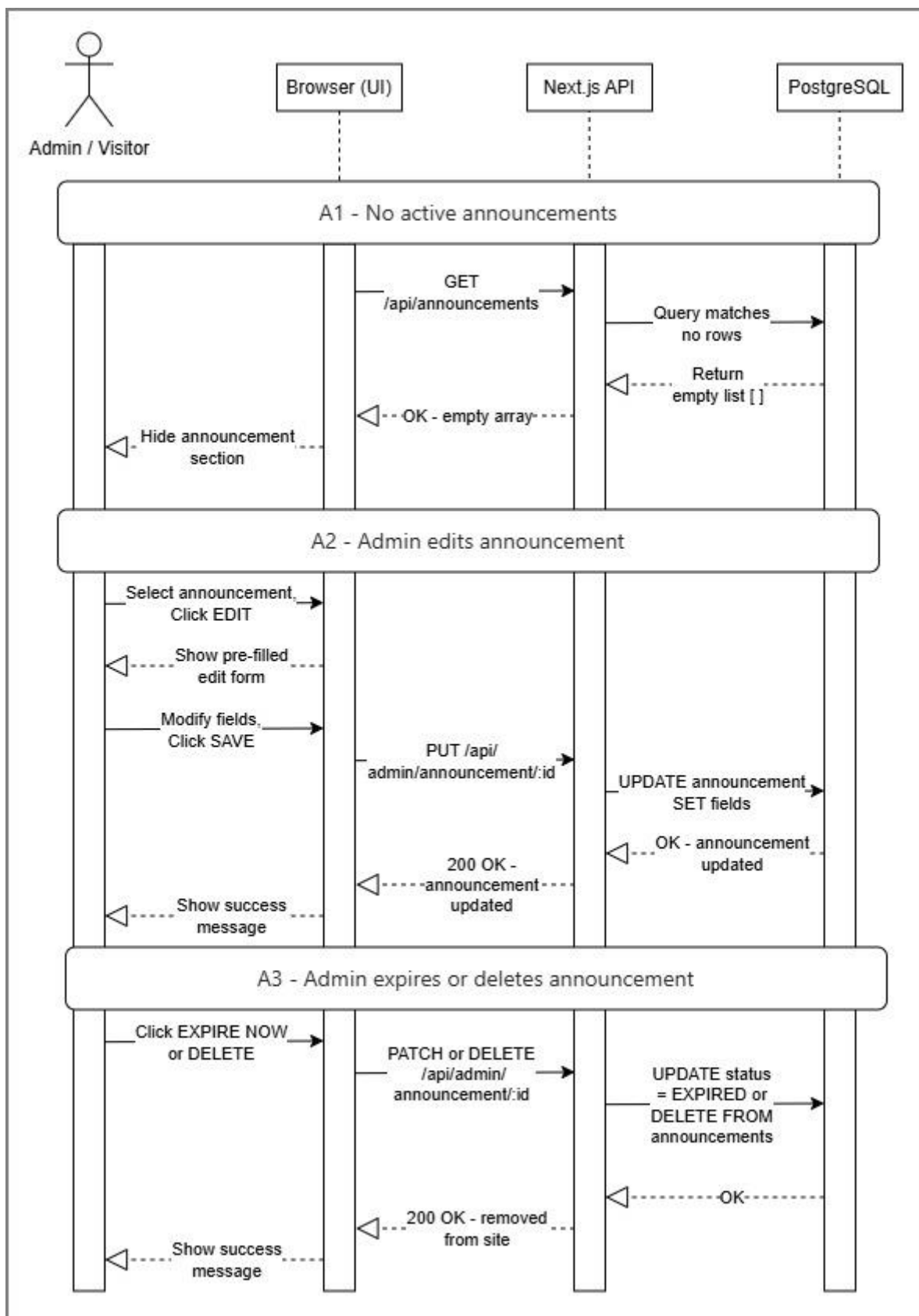
3.7.2 – Manage Announcements &amp; Promotions Alternative Flow Sequence Diagram
