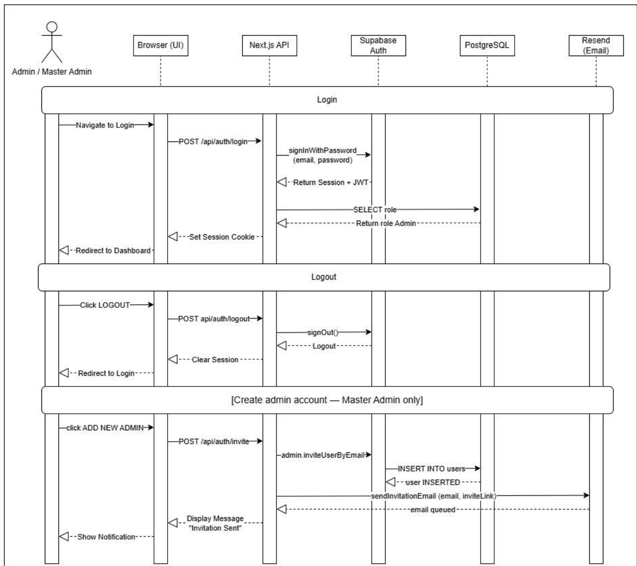
Figure 3.1.1 – User Access & Account Management Basic Flow Sequence Diagram
