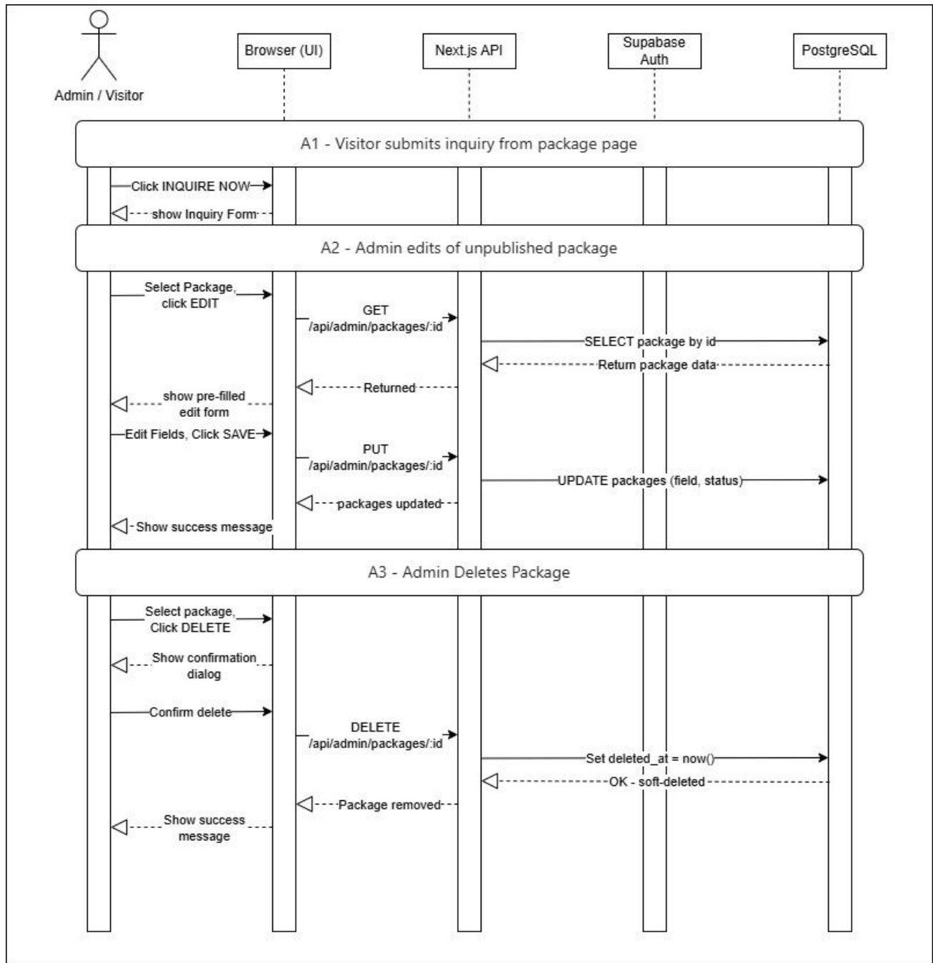
Figure 3.2.2 – Manage Packages Alternative Flow Sequence Diagram
