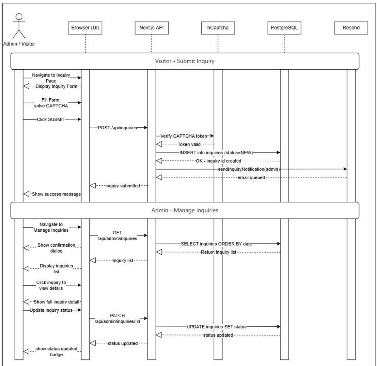
Figure 3.3.1 – Manage Inquiries Basic Flow Sequence Diagram
