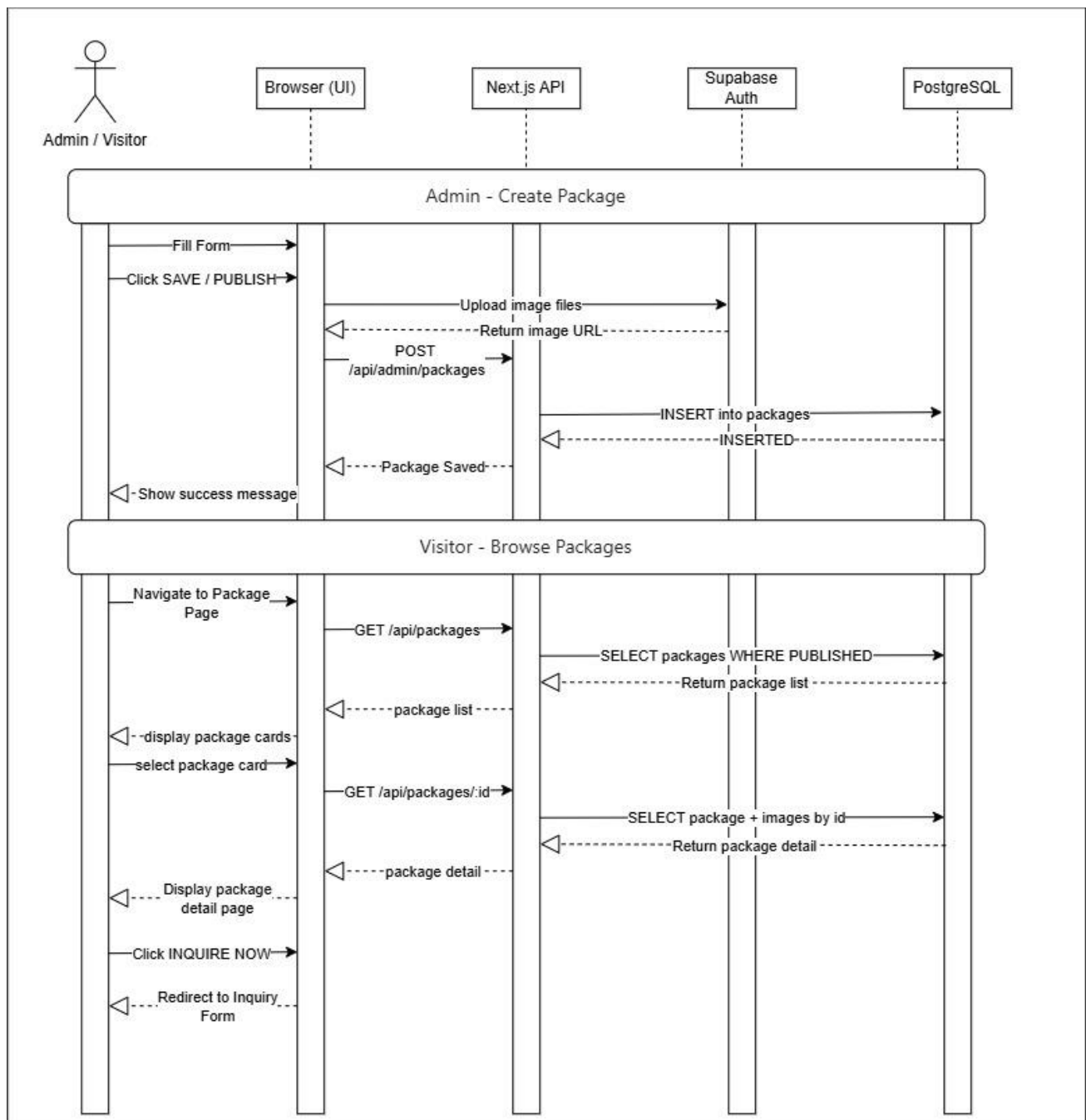
Figure 3.2.1 – Manage Packages Basic Flow Sequence Diagram
