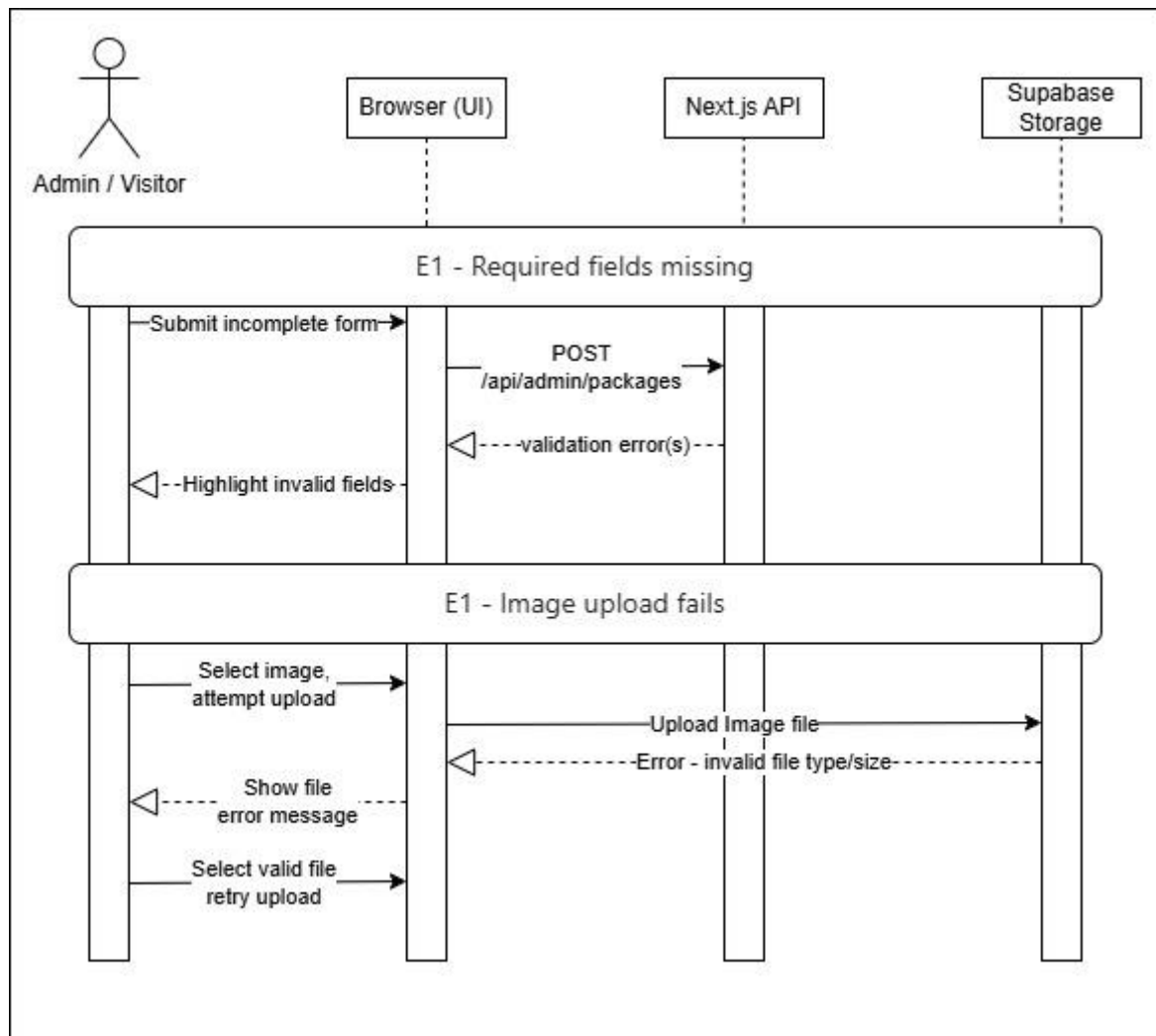
Figure 3.2.3 – Manage Packages Exception Flow Sequence Diagram
