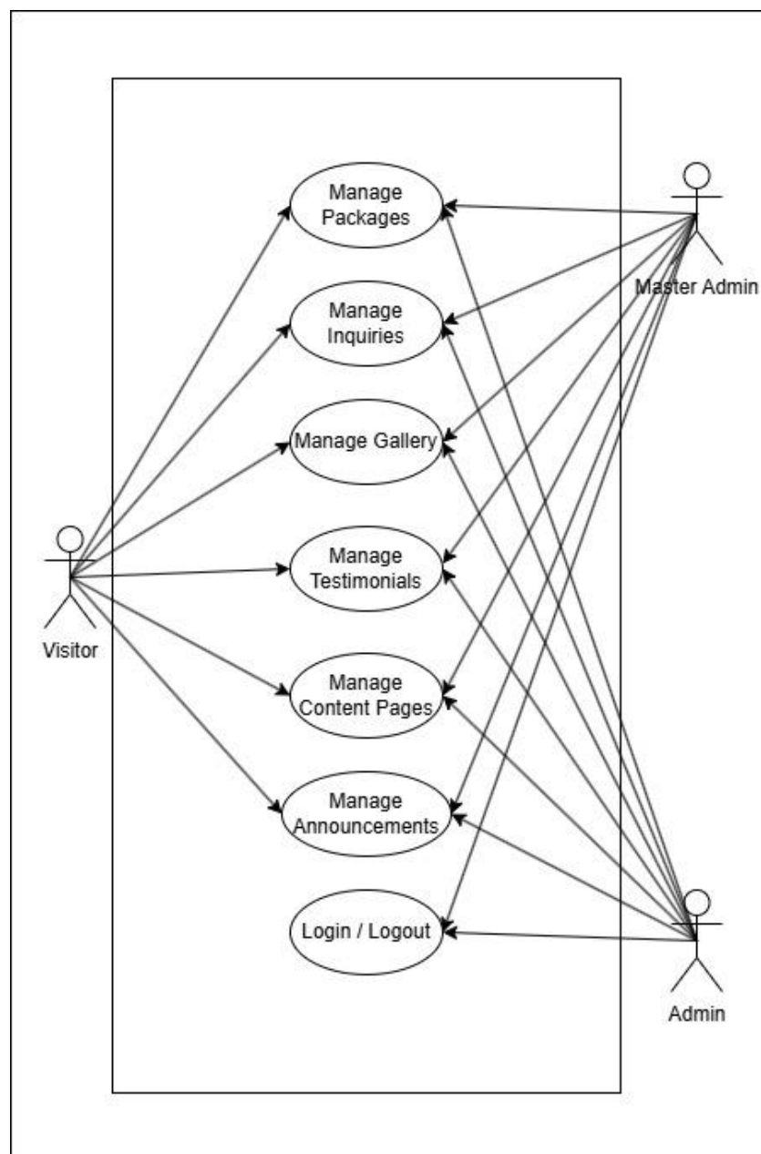
Figure 2.1 – Overall Use Case Diagram (MTT System)
