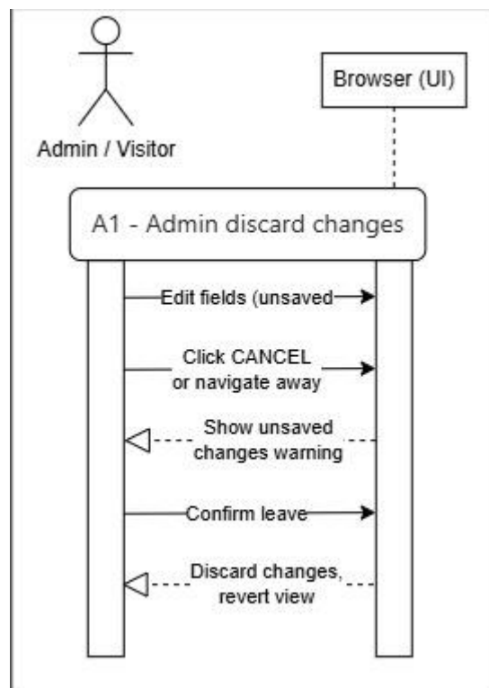
Figure 3.6.2 – Manage Content Pages Alternative Flow Sequence Diagram
