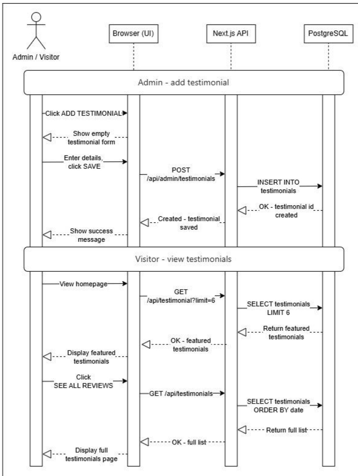
3.5.1 – Manage Testimonials Basic Flow Sequence Diagram
