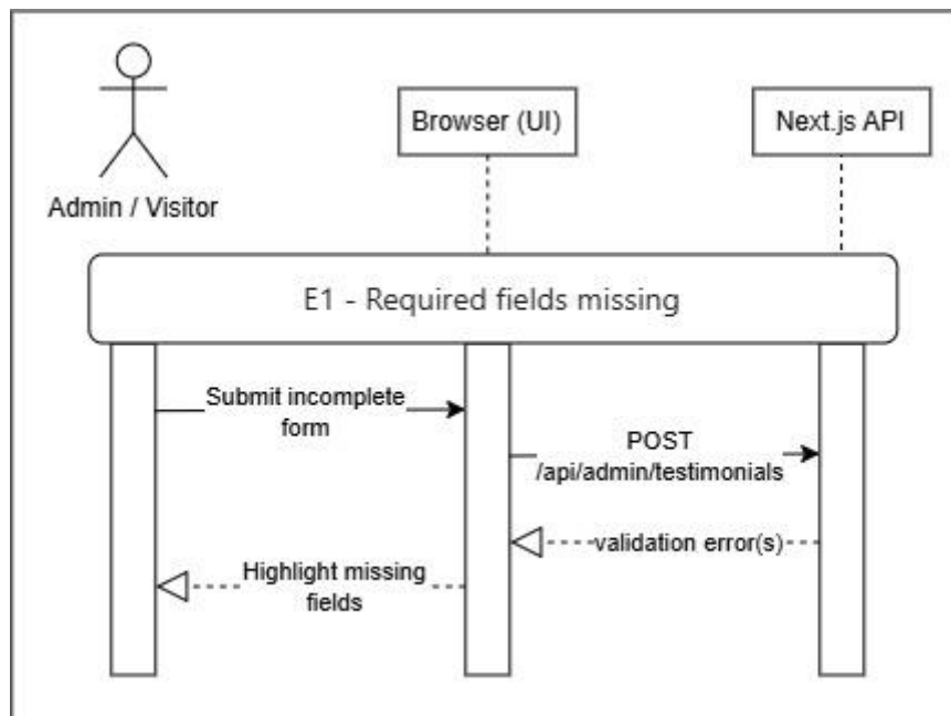
Figure 3.5.3 – Manage Testimonials Exception Flow Sequence Diagram
