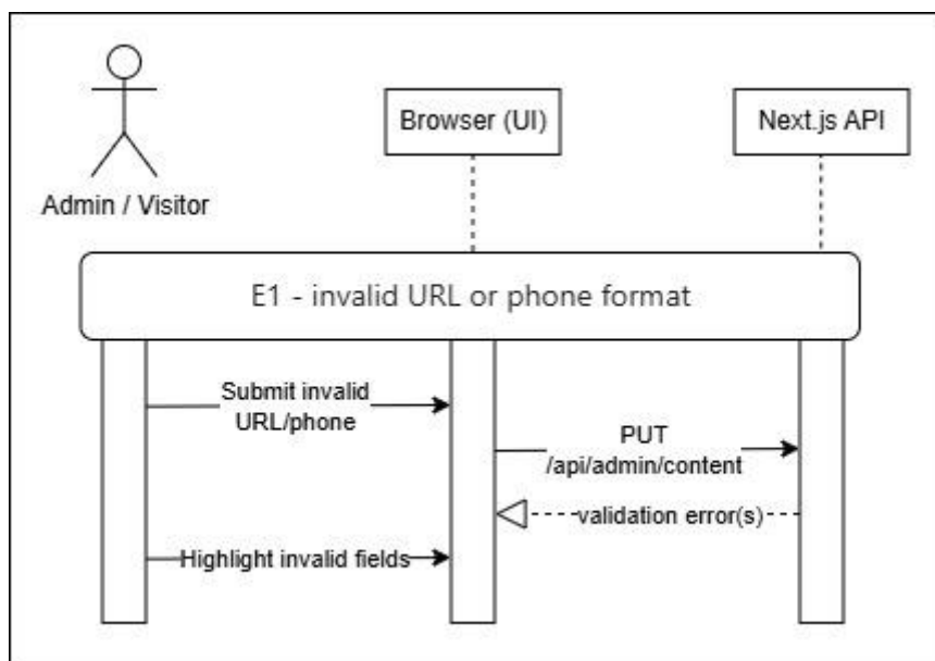
Figure 3.6.3 – Manage Content Pages Exception Flow Sequence Diagram
