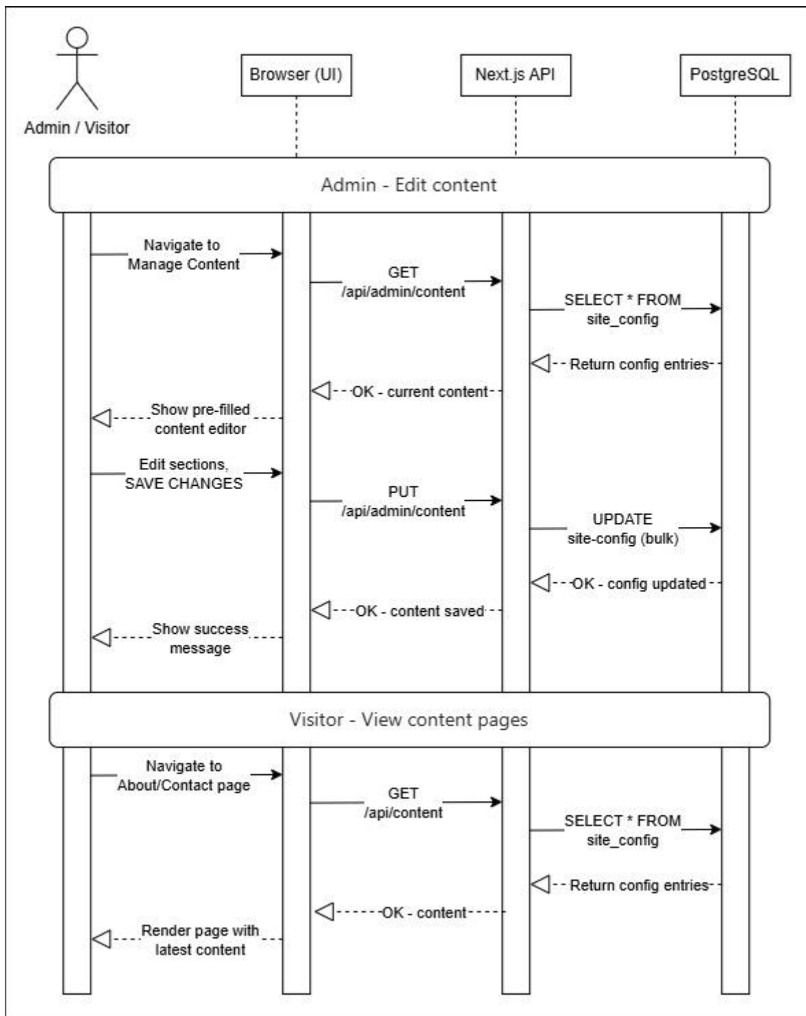
3.6.1 – Manage Content Pages Basic Flow Sequence Diagram
